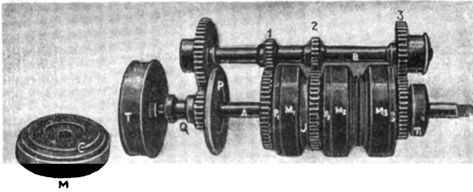
Transmission Parts, Showing Clutches in Place.
